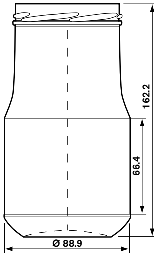
720 ml TO 77 Atlas #100340 Pallet Qty. 900 (L)
