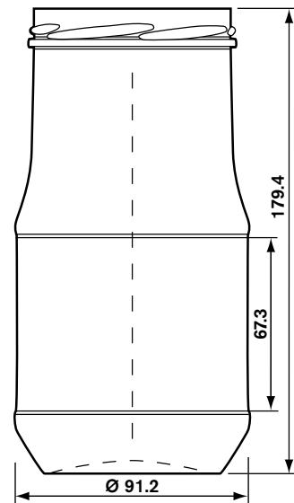
850 ml TO 82 Atlas #100157 Pallet Qty. 1,500 (H)
