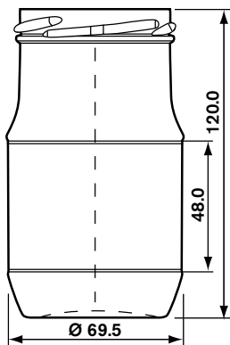
320 ml TO 63 Atlas #100326 Pallet Qty. 3,960 (H)
