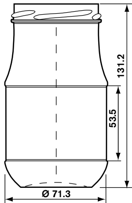
370 ml TO 63 Atlas #100135 Pallet Qty. 3,584 (H)
