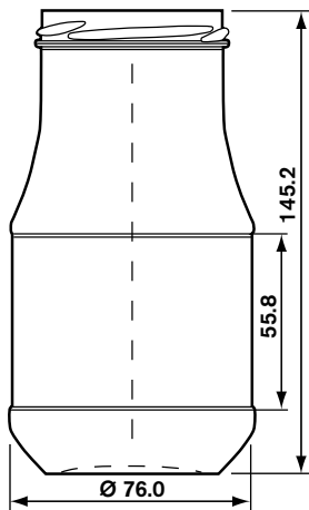
446 ml TO 63 Atlas #100280 Pallet Qty. 2,700 (H)
