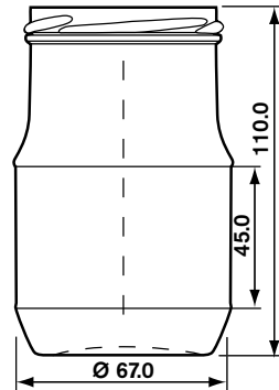
280 ml TO 63 Atlas #100127 Pallet Qty. 4,624 (H)
