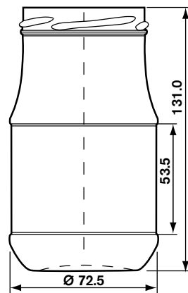
385 ml TO 63 Atlas #100552 Pallet Qty. 1,680 (L)
