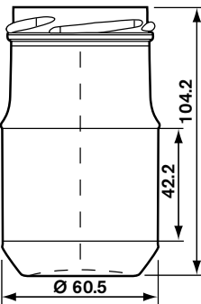
212 ml TO 58 Atlas #100130 Pallet Qty. 6,137 (H)
